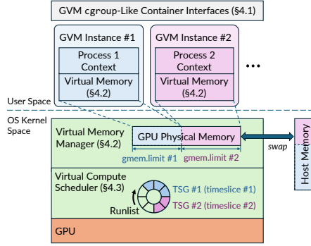
Figure 6: GVM design overview.
