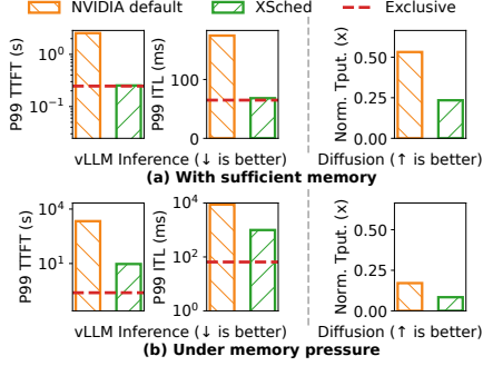
Figure 1: Performance of colocated vLLM and diffusion on an A100-40G GPU. (a) With sufficient memory. (b) Under memory pressure. the effects of SM sharing and swapping in this motivational study, we drive the applications with a synthetic request stream that maintains stable compute and memory pressure. The end-to-end evaluation in §6.3 instead uses a bursty production trace with the same application memory demands.
