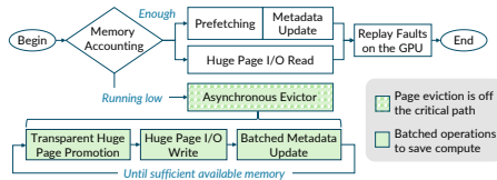
Figure 8: GVM’s page-fault handling path. GVM enforces per-container limits, uses huge-page-aware batching, and decouples eviction from the critical fault path.
