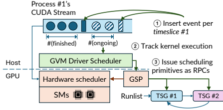
Figure 10: GVM's driver-hardware collaborative scheduling.
