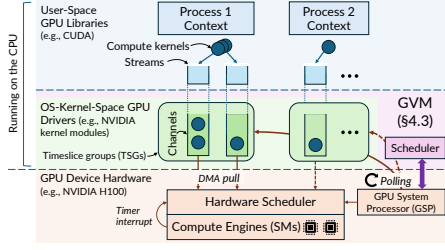
Figure 5: GPU compute scheduling hardware/software architecture.
